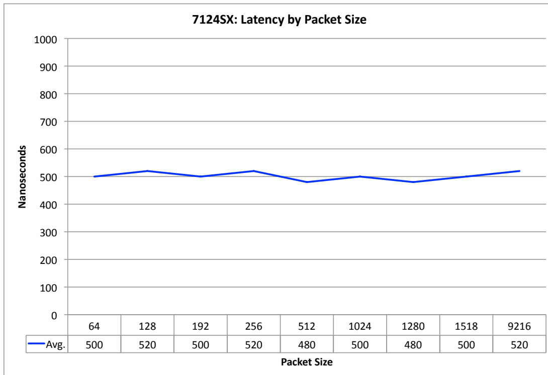
Arista 7124SX: Latency using RFC 2544 tests
