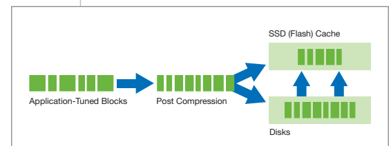
Figure 1: CASL Architecture
